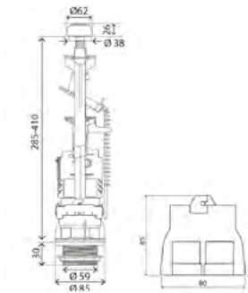
Univ. Dual flush valve • Dual flush mechanical action valve • Can be used with most popular WCs without dismantling tank • For all other WCs it is a universal system for models with a flush button of 16 and 50 mm • Laboratory tested flush system with all kinds of water • Up to 250.000 cycles guaranteed. • Slide and clip height adjustable overflow from 22 cm to 34 cm • Enables practical and effective adjustment of overflow in all manner of tanks • Anti-flooding overflow draining up to 20 L per minute • 5 year warranty • Made in Europe
