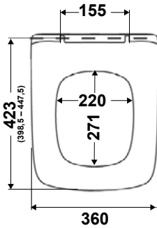
Cuadro Universal Seat • Up to 100,• Works with Formentera non-compact floor mounted WCs and other square models of any brand • D-shaped seat • Slim design • Made of UF (Urea 131.5 Thermoset) • Crack and scratch resistant • No colour variation over time • Soft-close system with a useful life of over 100,000 cycles • 3 year warranty • Made in Europe 000 open and close cycles
