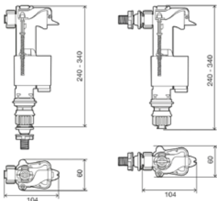
Tank filling valve – univ. use • A single reference for all side and bottom entry WCs • Long brass 3/8" thread that can even be installed in older WCs • More silent and resistant to pressure surges due to rubber reducer • Silent close • Built-in filter that can be cleaned without dismantling inlet pipe • Fast regulation system with no need for tools • Takes up less space in tank. Height adjustment • No blockages even if not correctly installed • Mounted to water connection with ¼ turn • 5 year warranty • Made in Europe
