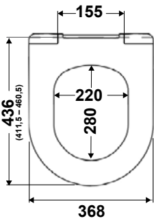
Rondo Universal Seat • Works with Inca, Manacor, Nexoas and other brand rounded models of floor mounted WCs • D-shaped seat • Slim design • Made of UF (Urea 131.5 Thermoset) • Crack and scratch resistant • No colour variation over time • Soft-close system with a useful life of over 100,000 cycles • 3 year warranty • Made in Europe
